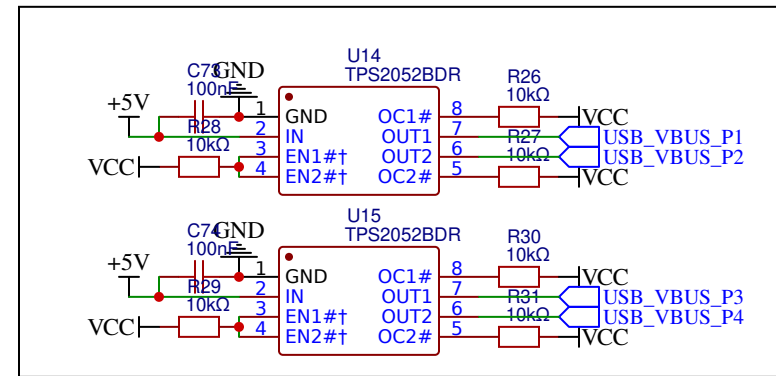
Short Prevention Chips (USB 2.0)
