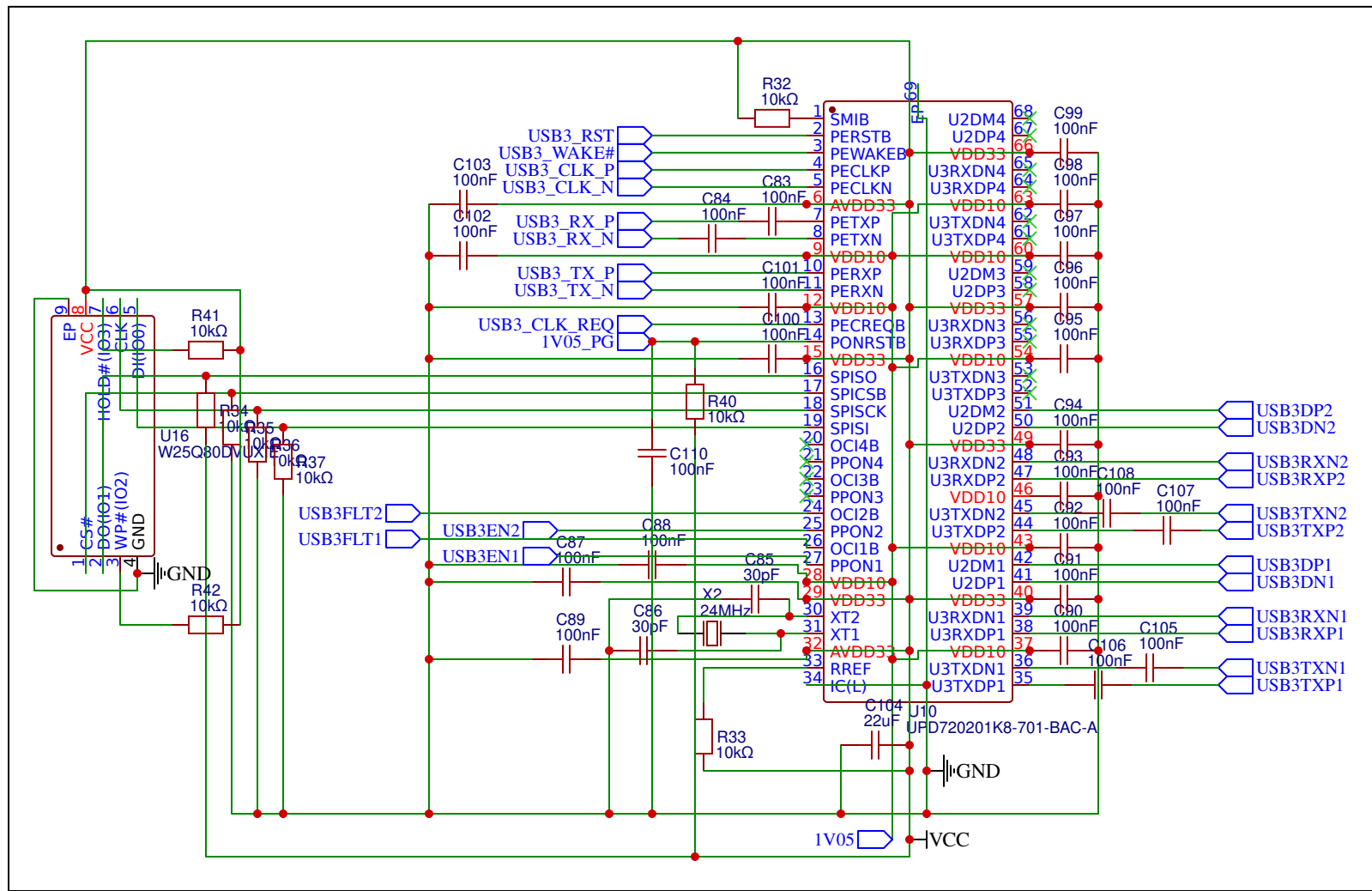
USB 3.2 Controller
