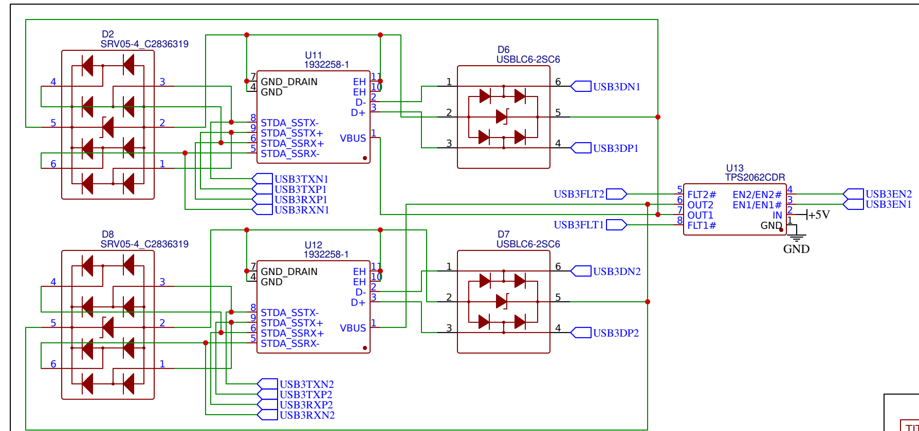
USB 3.2 Ports and TVS Protection
