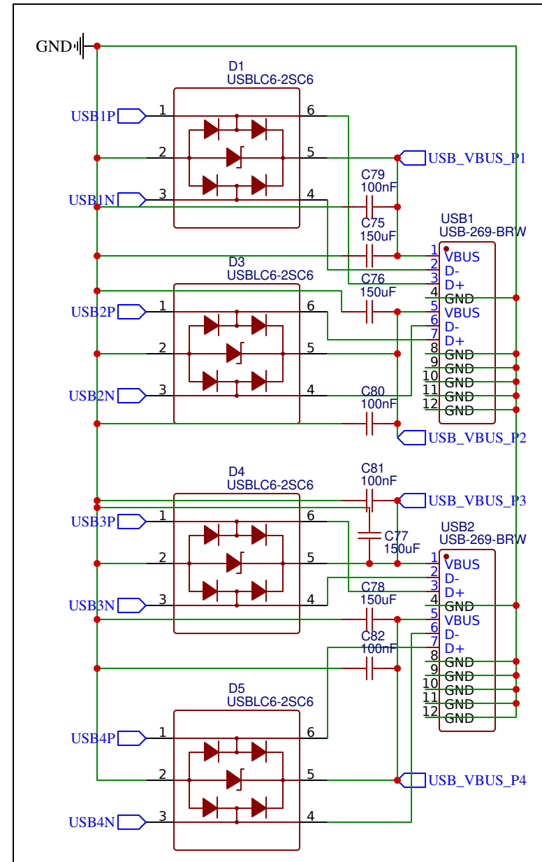
USB 2.0 Ports & TVS Protection
